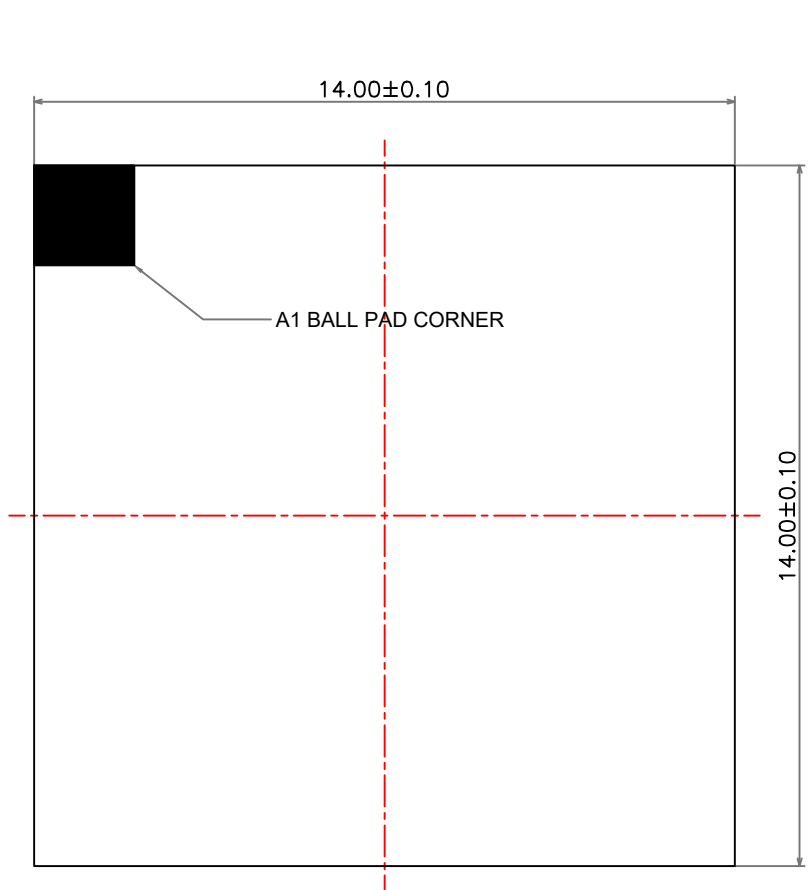
TOP VIEW
